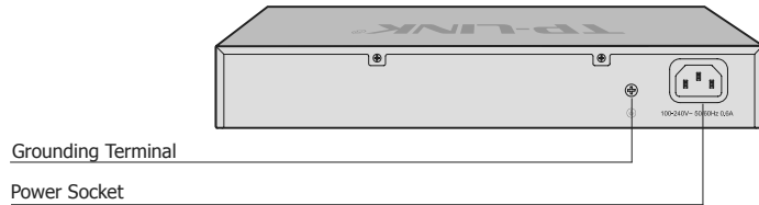
Figure 1-10 Rear Panel of TL-SG1008
