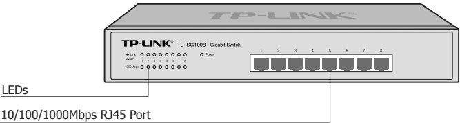
Figure 1-6 Front Panel of TL-SG1008
