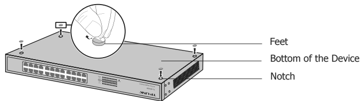
Figure 2-1 Desktop Installation
