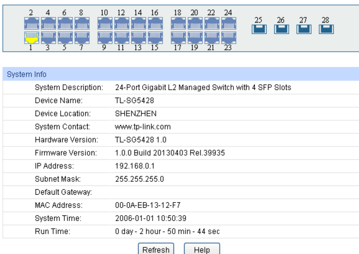
Figure 4-1 System Summary
